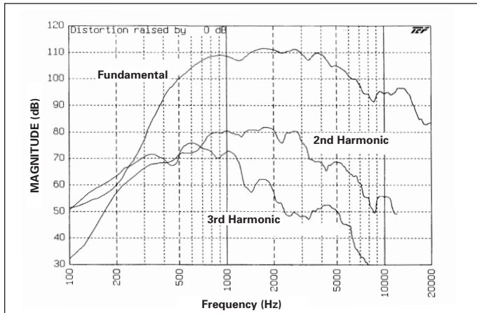
AP-15TU(C) (Harmonic Distortion - 1.5 watts @ 1 meter)
